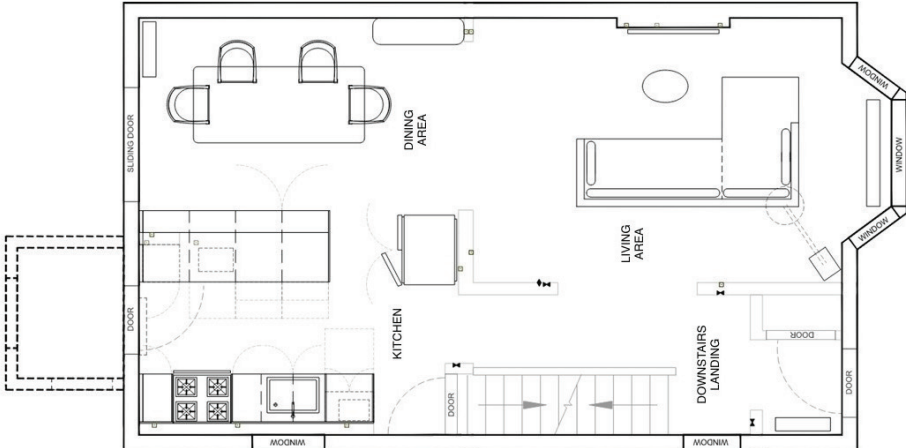
MAIN LEVEL
