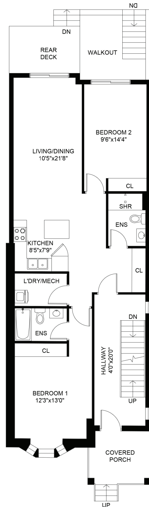
MAIN FLOOR PLAN
