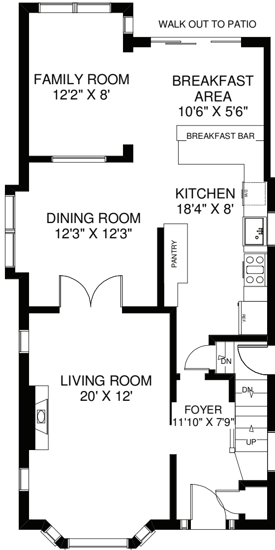
MAIN FLOOR APPROXIMATELY 950 SQ FT
