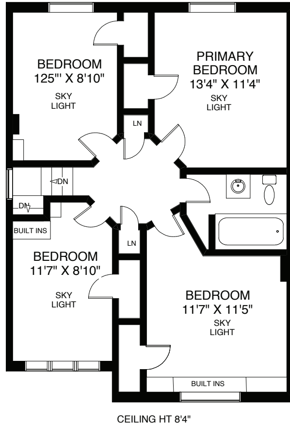
SECOND FLOOR APPROXIMATELY 790 SQ FT
