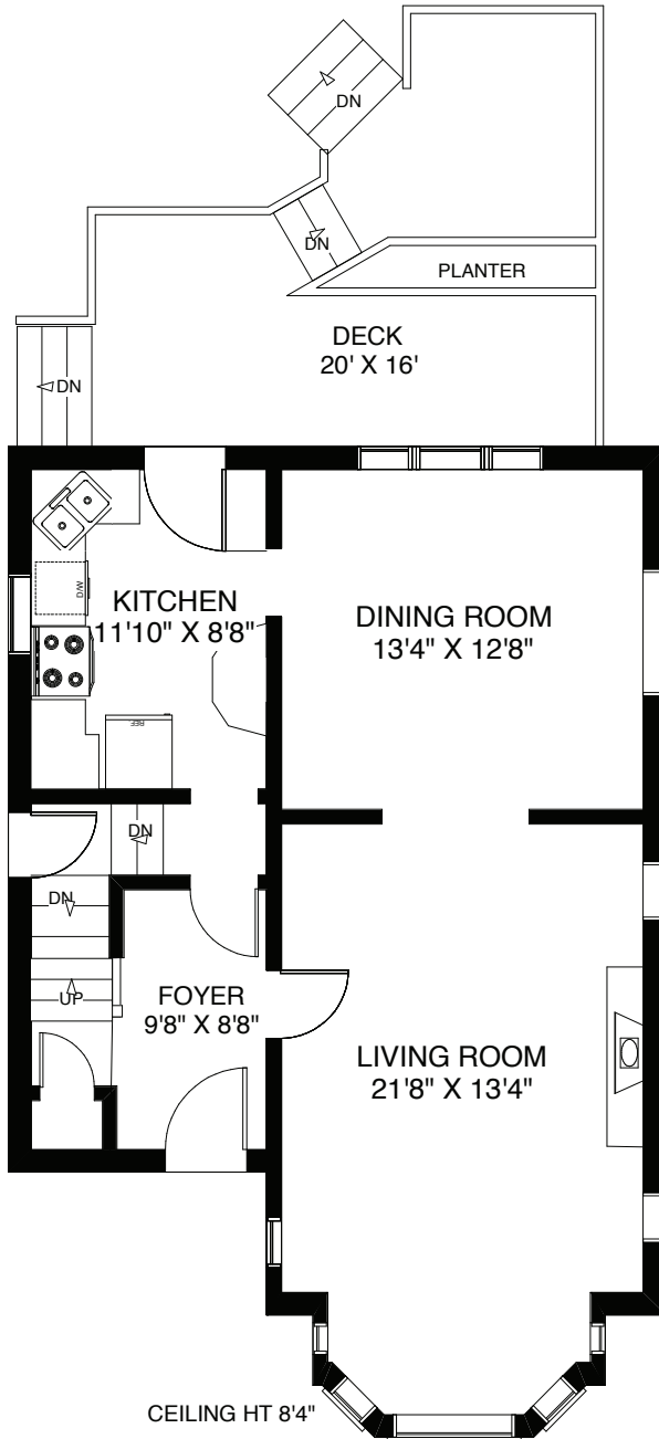
MAIN FLOOR APPROXIMATELY 760 SQ FT
