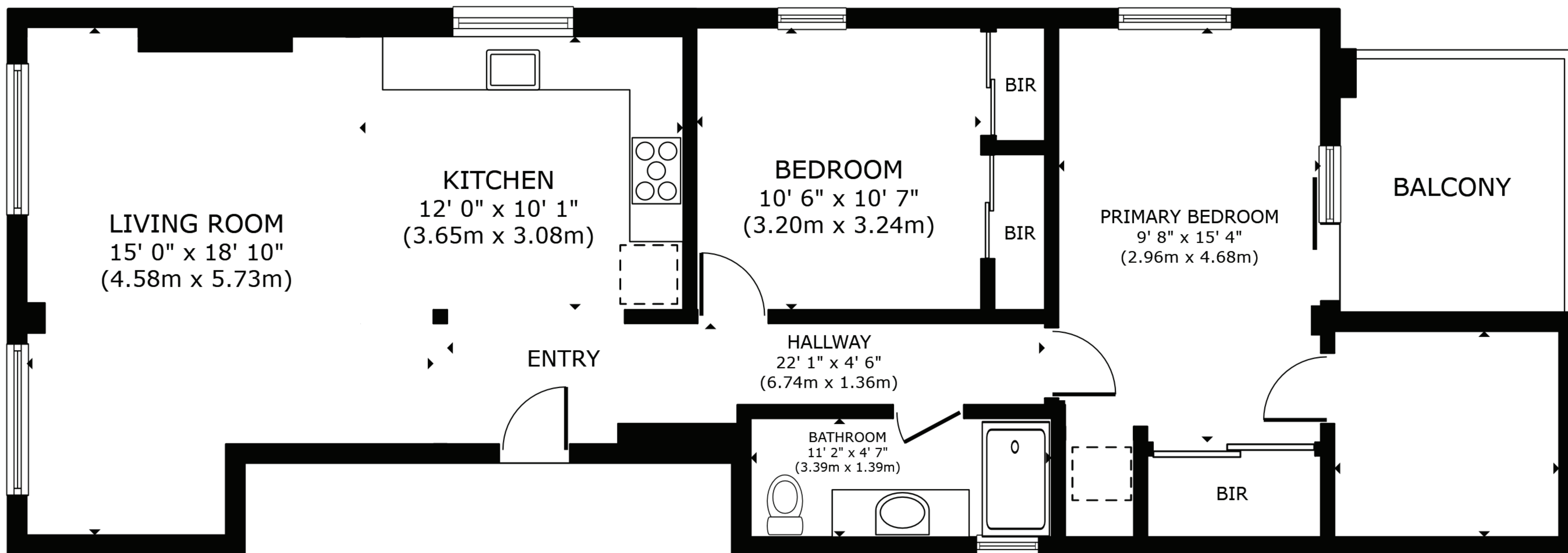
FLOOR PLAN
