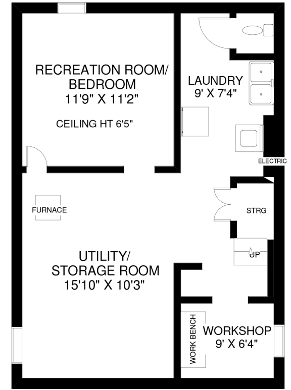
LOWER FLOOR APPROXIMATELY 680 SQ FT
